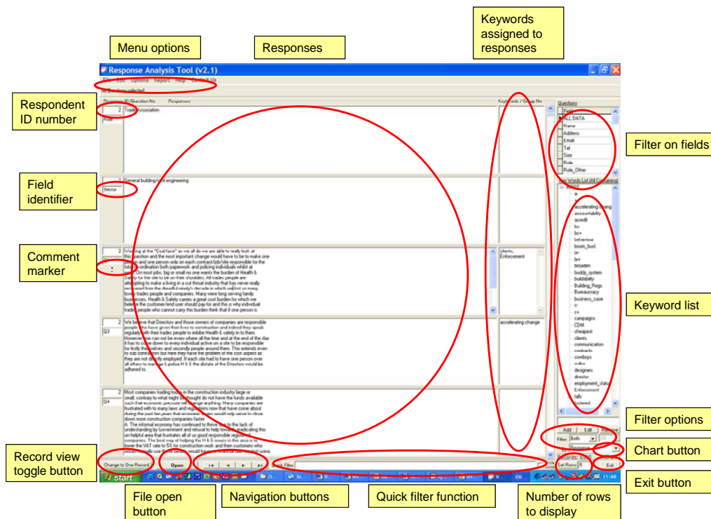
Figure 6 Response Analysis Tool user interface
